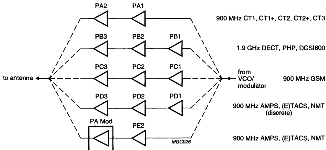
Fig.3 Typical power amplifier section for cordless and cellular phones
